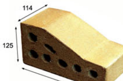
Kerb 8SF359-15-KERB
